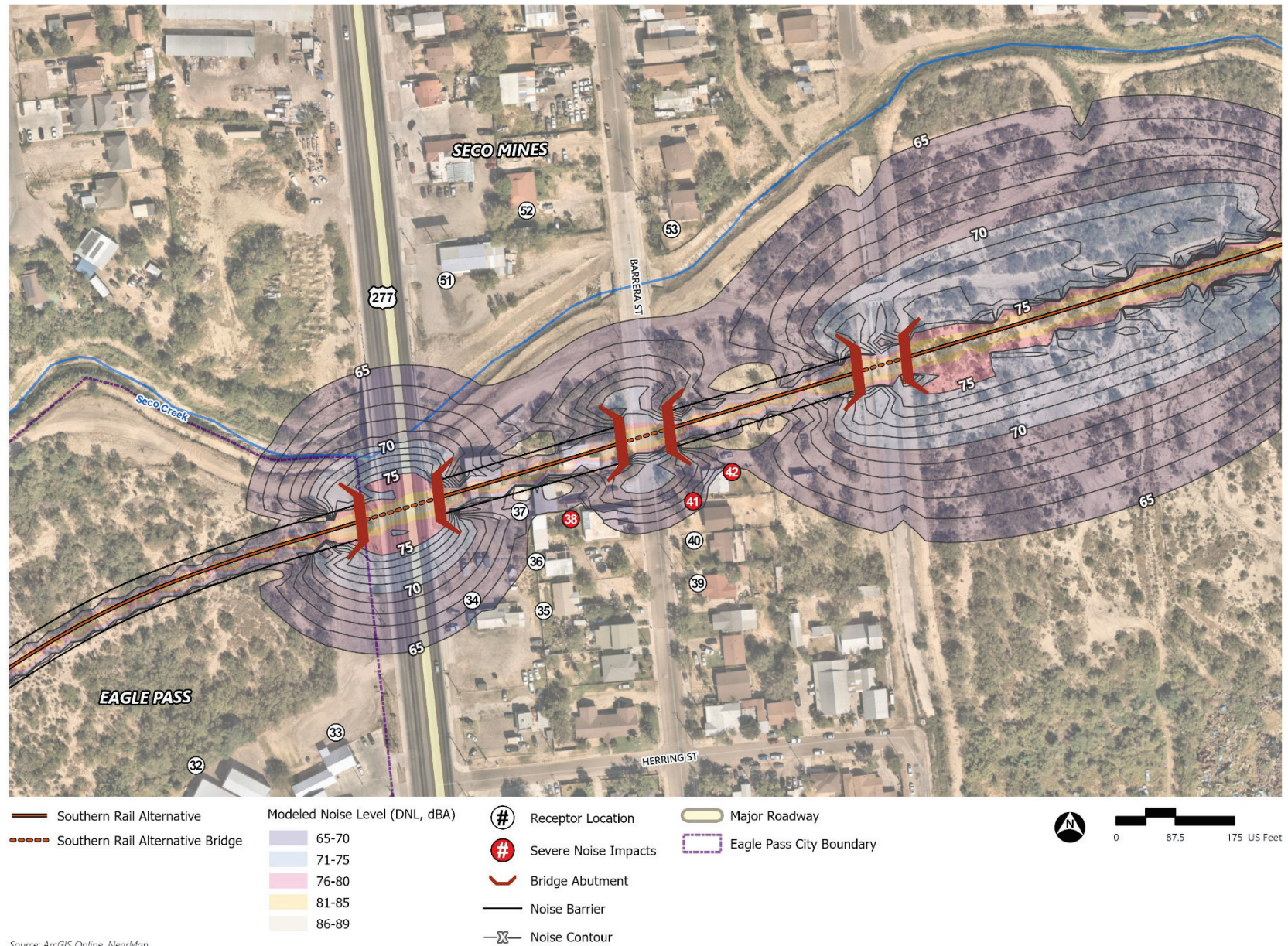
Figure G-5. Southern Rail Alternative Noise Contours with GER's Proposed Noise Barrier Design
